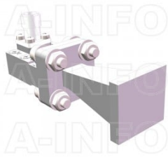
LB-28-10-C-2.4FSPO Standard Gain Horn Antenna 26.5-40GHz 10dB Gain 2.4mm Female
