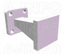
LB-28-10-ASPO Standard Gain Horn Antenna 26.5-40GHz 10dB Gain Rectangular Waveguide Interface
